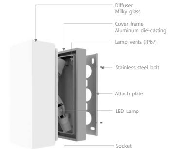
_ BRICK BRACKET LIGHT EXPLODED VIEW
